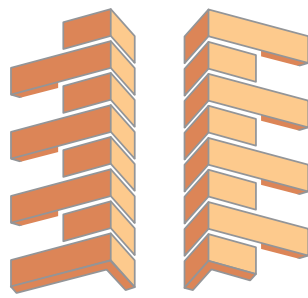
Left & right window reveal
