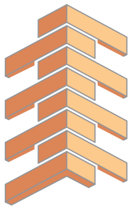
90° external return
